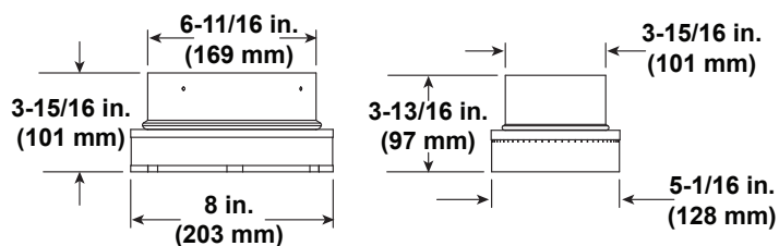
SLP-2DVP Adapter
